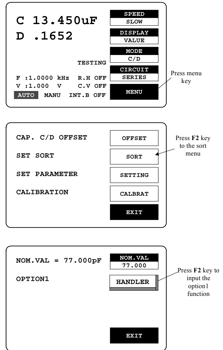
Figure 8-1.: OPTION 1 (BIN FUNTIONS) setting
