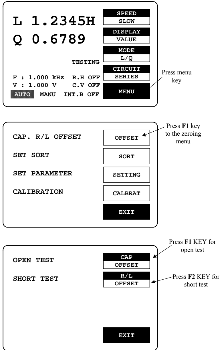
Figure 4-1: Summary of zeroing menu
