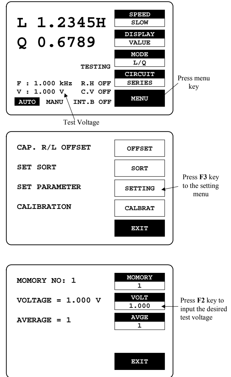
Figure 4-10. Programming of test voltage.
