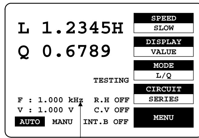
Figure 4-9. Inputs of test frequency
